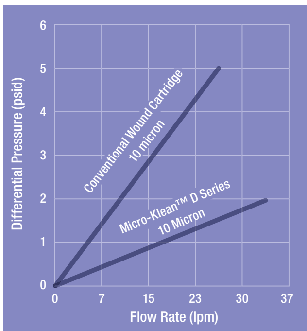
Graph 1 – Flow Comparison
